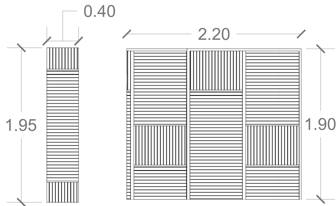
Fence Panel Details For Side Elevation
